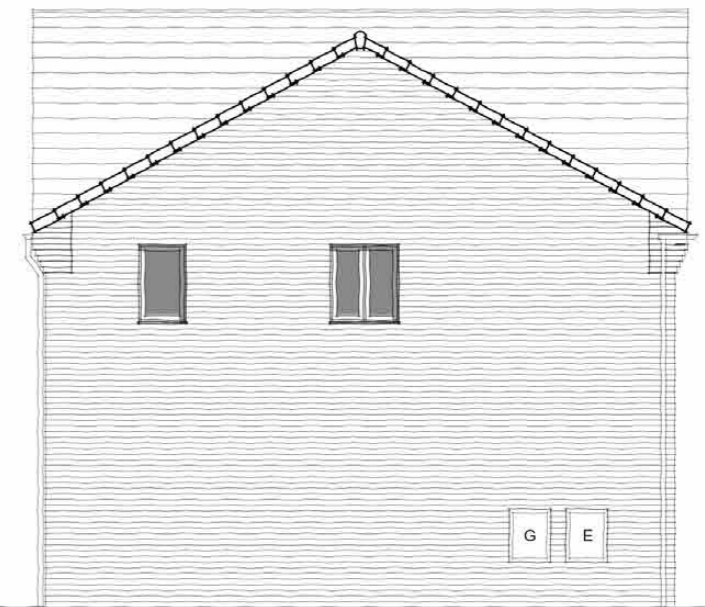
Side Elevation Cherry
