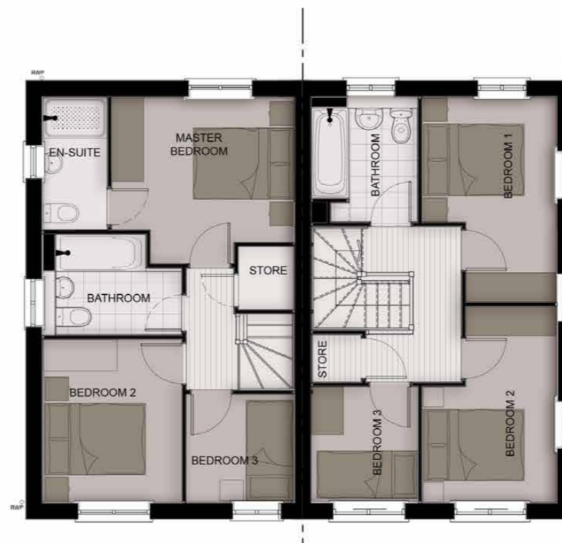
First Floor Plan Cherry
